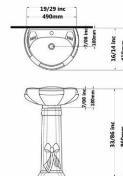
PLUTO Washbasin With Full Pedestal
