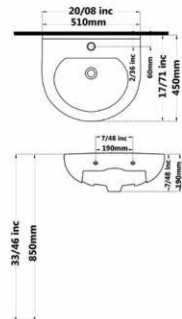
AY Washbasin With Full Pedestal
