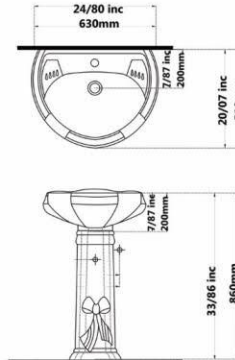
PLUTO Washbasin With Full Pedestal
