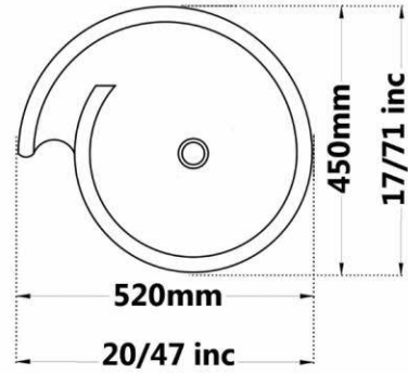
GALAXY Countertop Basin Circle Without Tap Hole
