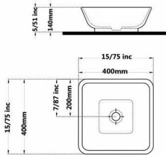
SATRON Countertop Basin Square With Tap Hole
