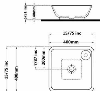
SARINA Countertop Basin Square With Tap Hole
