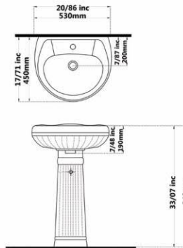
ZOHREH Washbasin With Full Pedestal
