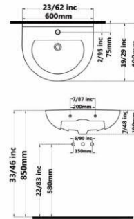
AY Washbasin With Full Pedestal
