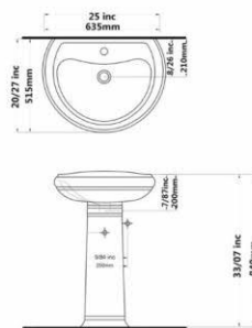
ATAROD Washbasin With Full Pedestal
