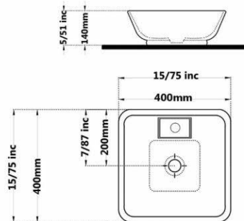
SARINA Countertop Basin Square With Tap Hole
