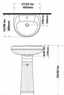
ZOHREH Washbasin With Full Pedestal
